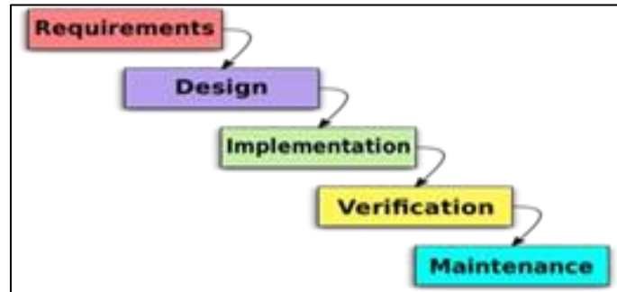
Fig 1: Waterfall method
